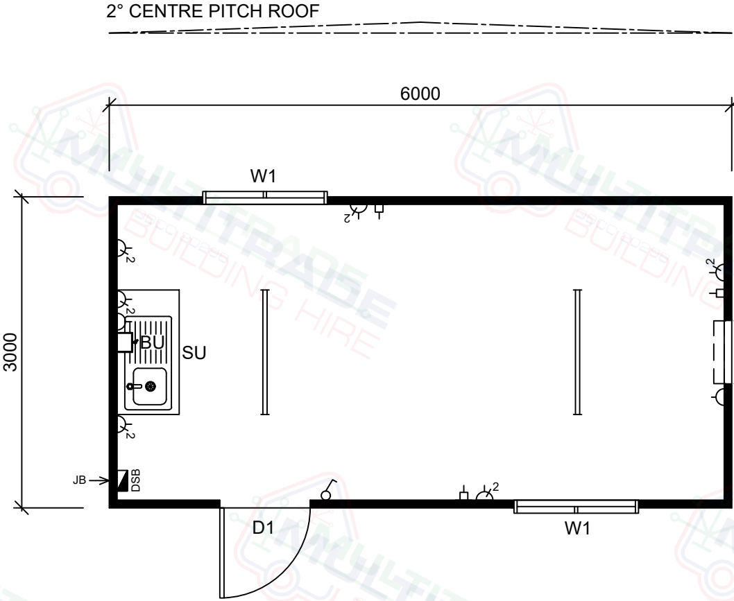
6.0x3.0m Crib Room - Floor Plan
